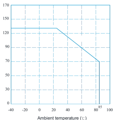
Turn off time Vs. Ambient temperature
