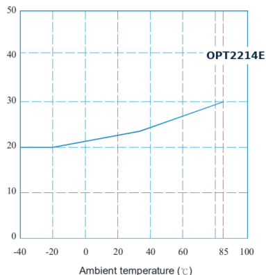
On resistance Vs. Ambient temperature
