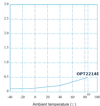
LED turn off current Vs. Ambient temperature
