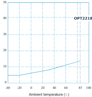
LED operate current Vs. Ambient temperature
