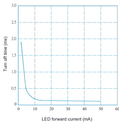
LED forward current Vs. Operate (OFF) time characteristics
